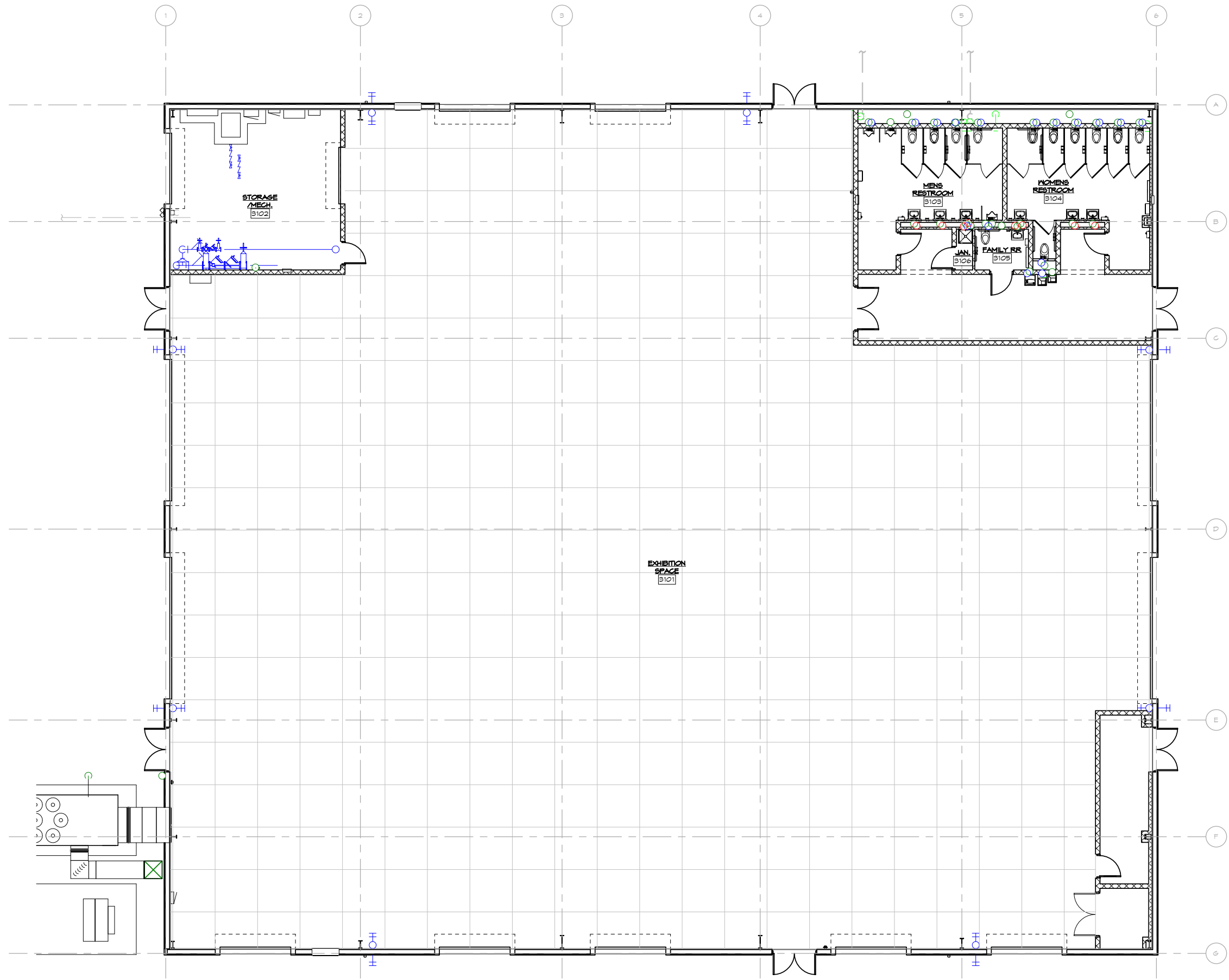
BUILDING #3 - FLOOR PLAN GRID SHOWN MEASURES 6'-0" X 6'-0"
